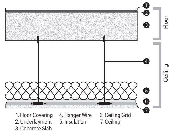
Figure 4: Illustration of Structure for STC/IIC Testing
